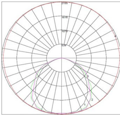
MHT-GRW-100E
